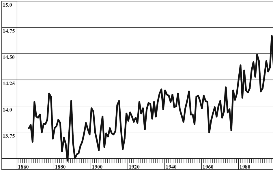
Figure 10 Average temperature at the Earth's surface, 1860-1998
