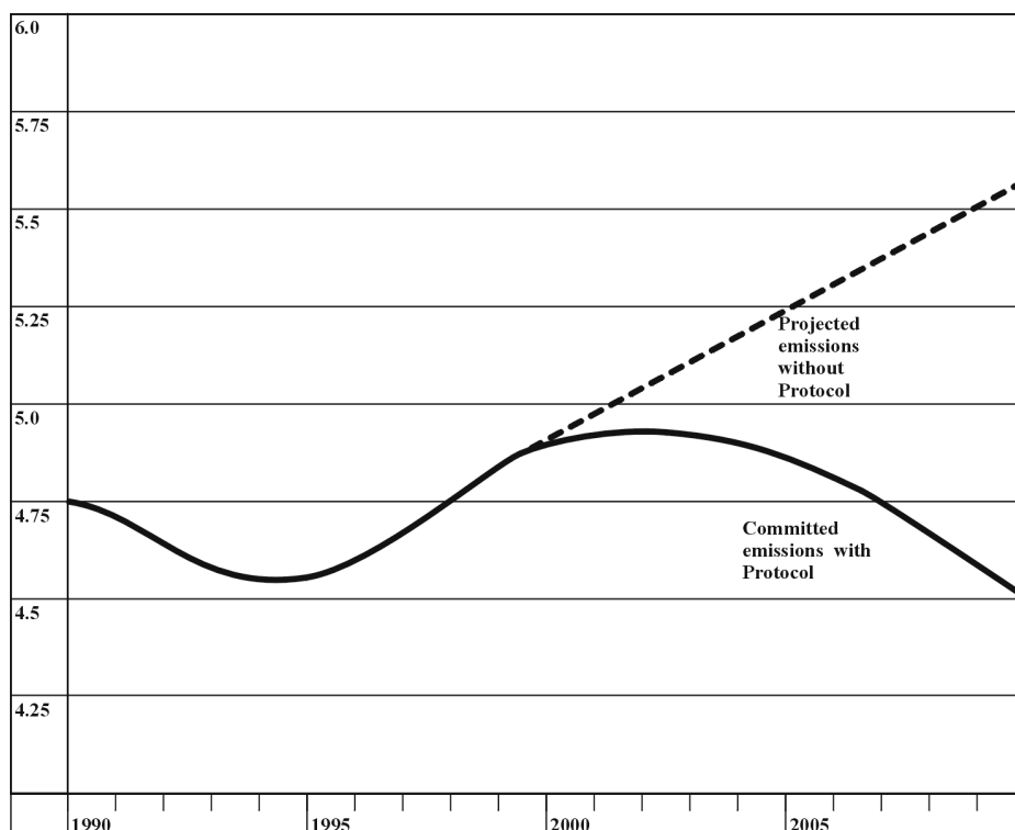
Figure 12 Projected impact of the Kyoto Protocol on emissions of greenhouse gases
